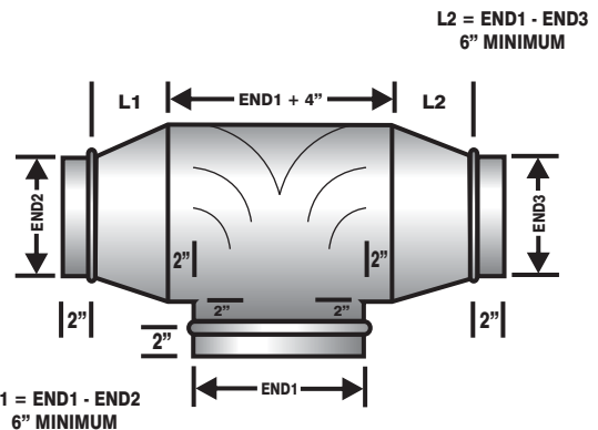
REDUCING BULL HEAD TEE
