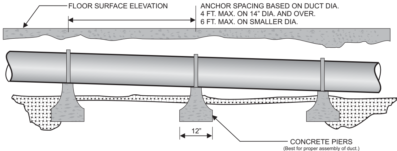
TYPICAL ANCHORAGE OF DUCTS TO BE ENCASED IN CONCRETE
