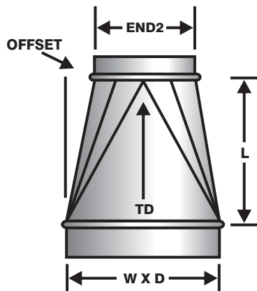
RECTANGLE TO ROUND
