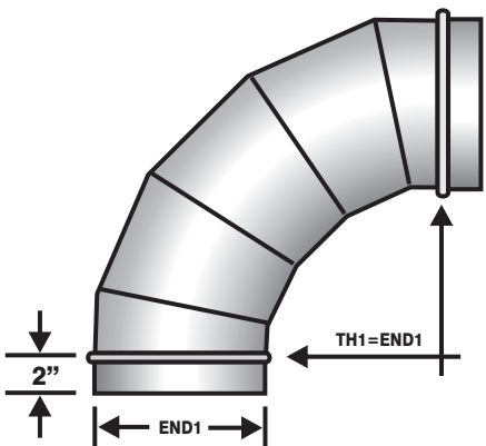
90° 5-PIECE GORE-LOCKED ELBOW
