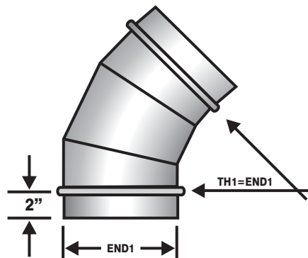
45° 3-PIECE GORE-LOCKED ELBOW
