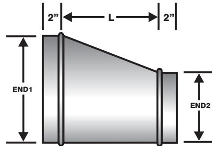
ECCENTRIC REDUCER
