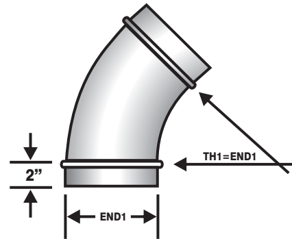
45° DIE STAMPED ELBOW 3" DIA. THRU 12"
