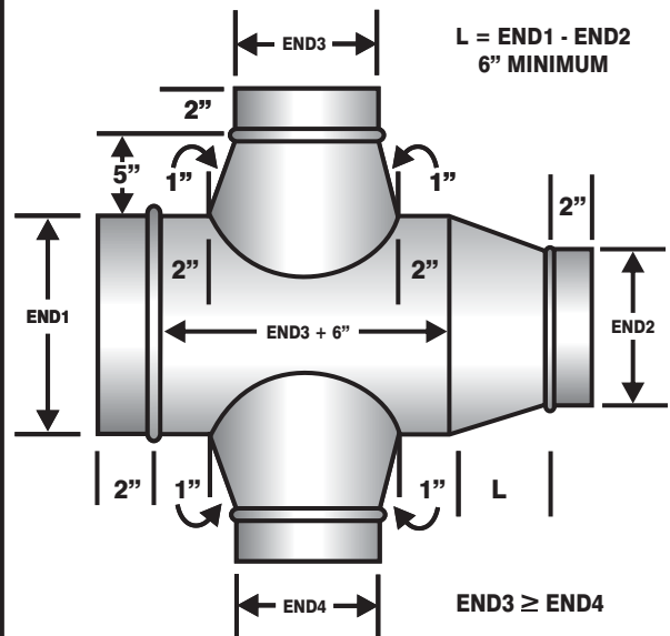
REDUCING CONICAL TEE CROSS
