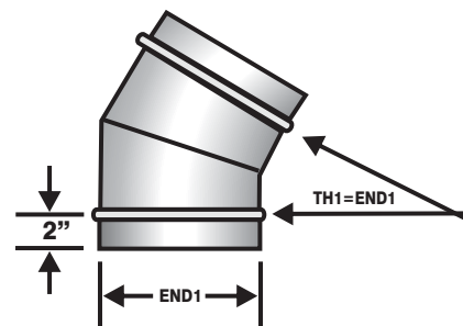
15° & 30° 2-PIECE GORE-LOCKED ELBOW
