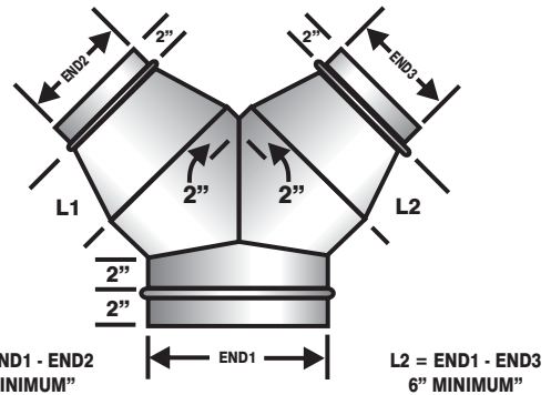
REDUCING Y BRANCH
