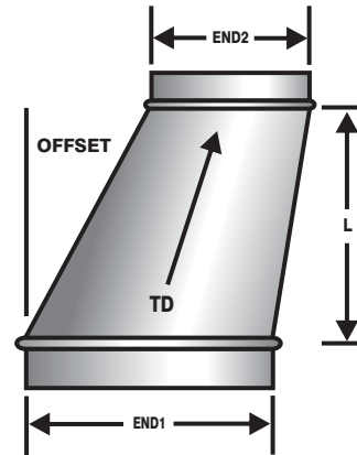
ROUND TO ROUND
