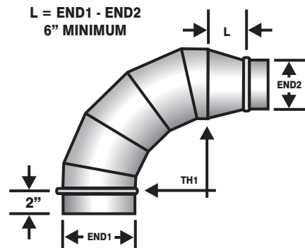
90° 5-PIECE ELBOW WITH REDUCER
