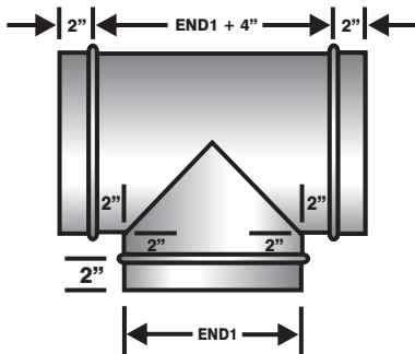
BULL HEAD TEE
