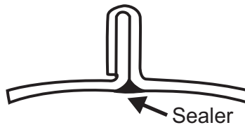
GORE-LOCKED SEAM
