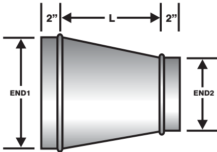
CONCENTRIC REDUCER
