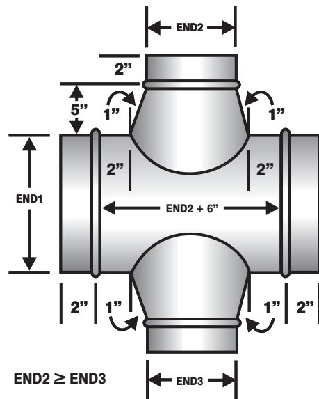
CONICAL TEE CROSS
