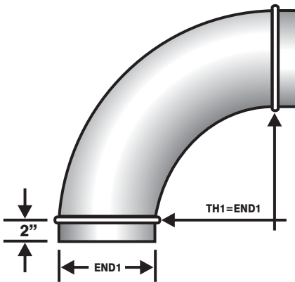
90° DIE STAMPED ELBOW 3" DIA. THRU 12"
