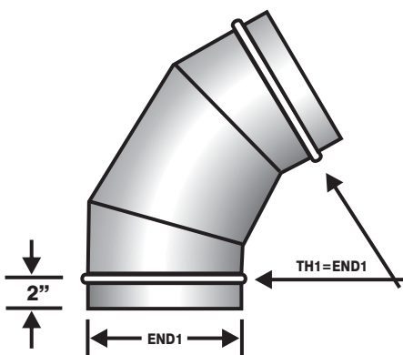
60° 3-PIECE GORE-LOCKED ELBOW
